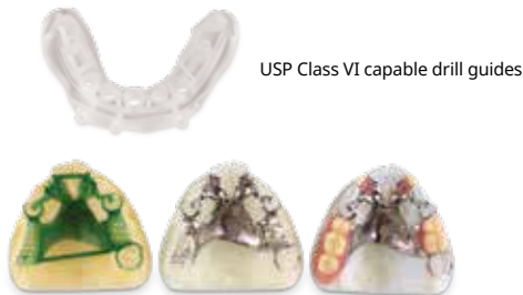
Partials and working models printed on the Projet MJP 3600 Dental
